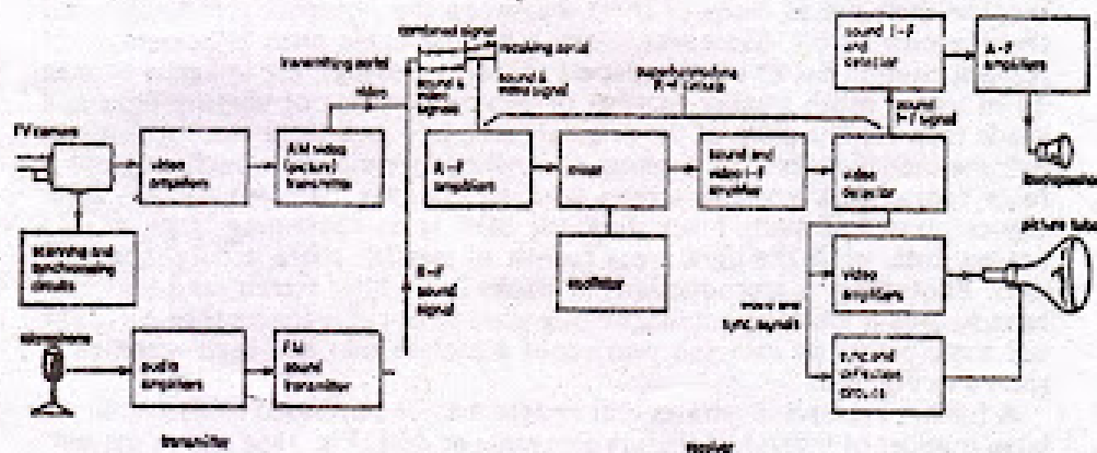
Fig. 187. Simplified diagram of television system
